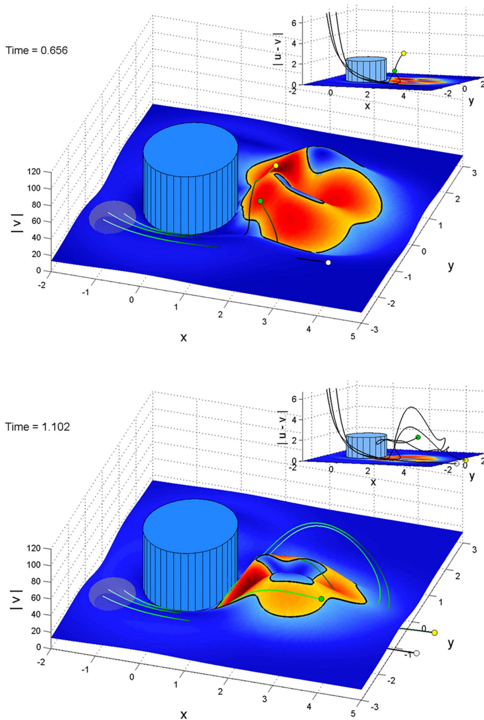
FIG. 2. (Color online) Global convergence of neutrally buoyant particles to the slow manifold M_\epsilon , interrupted by regions of divergence along the slow manifold. The repelling domain on the slow manifold, encircled by the black solid curves (red regions online), satisfies formula (13).
